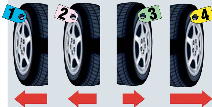
Tires are tagged and positioned on the vehicle to provide the least amount of vehicle pull and obtain the best straight-steering stability.
